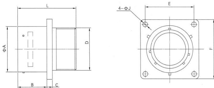
Wall mounting receptacle (MS3110R)
