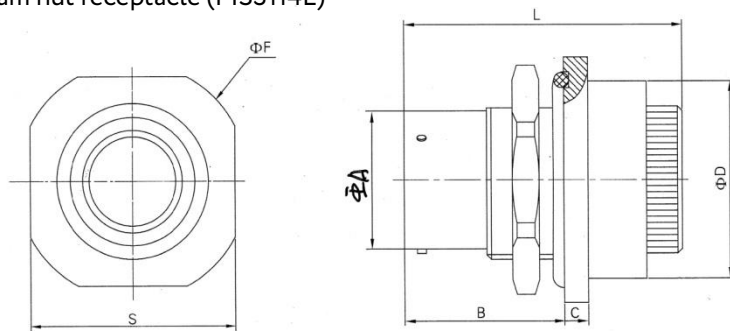
Jam nut receptacle (MS3114E)
