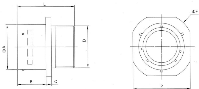
Cable connecting receptacle (MS3111R)
