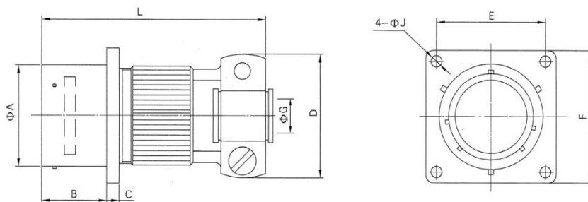
Wall mounting receptacle (MS3110F)
