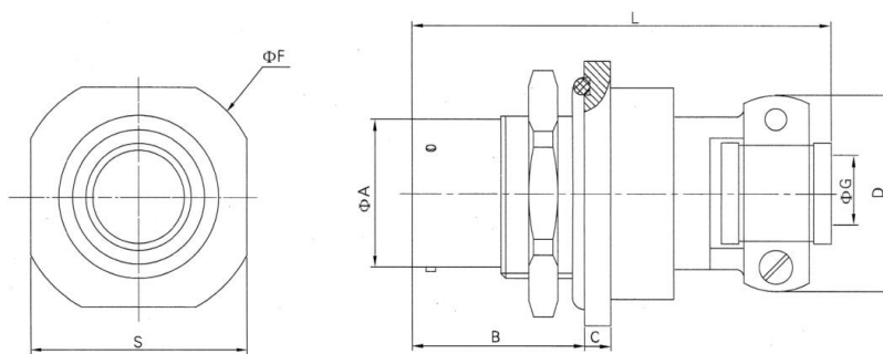
Jam nut receptacle (MS3114F)
