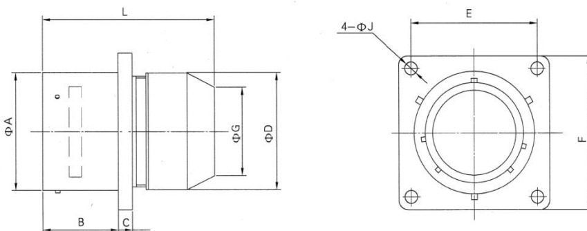
Wall mounting receptacle (MS3110P)
