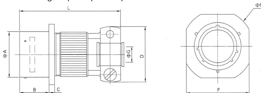
Cable connecting receptacle (MS3111F)
