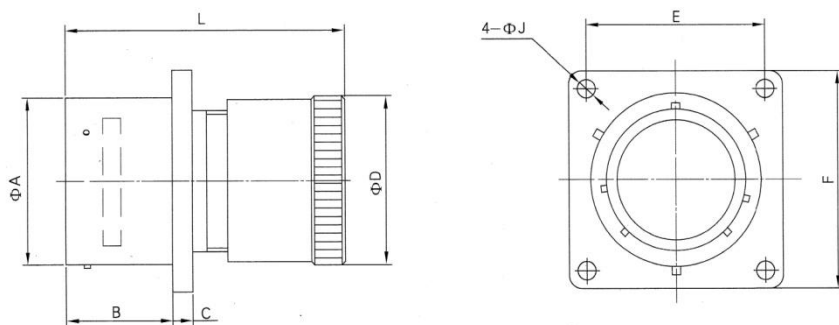
Wall mounting receptacle (MS3110E)
