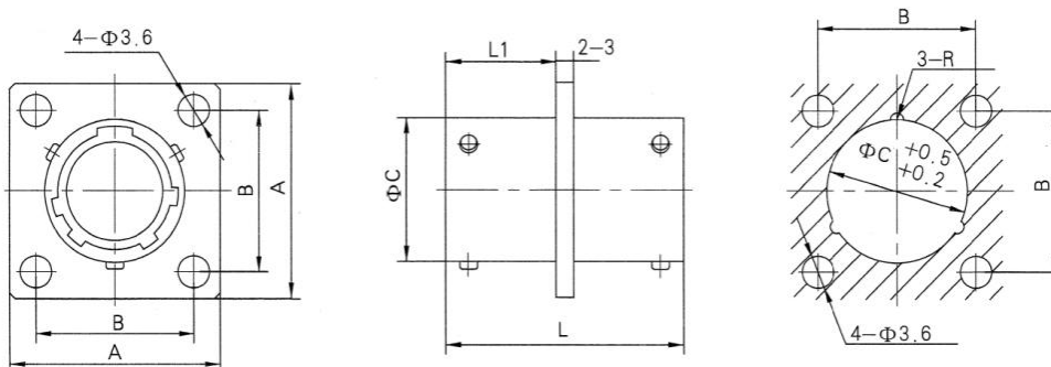
Thru bulkhead receptacle (MS3117P)
