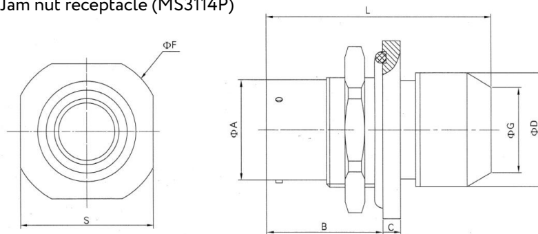
Jam nut receptacle (MS3114P)
