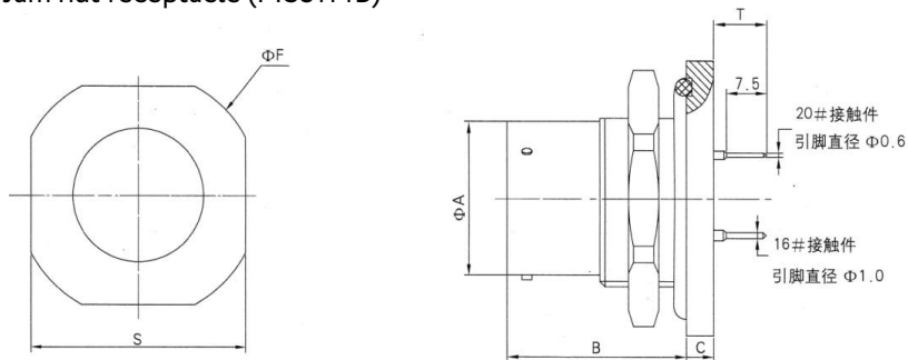
Jam nut receptacle (MS3114B)
