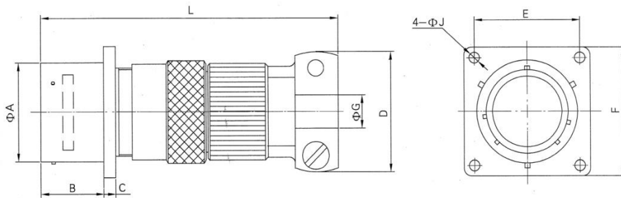
Wall mounting receptacle (MS3110J)
