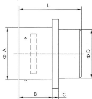
Box square flange receptacle (MS3112E)
