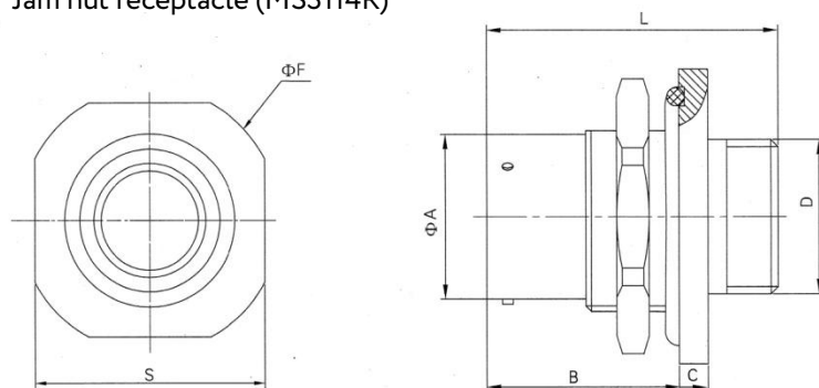
Jam nut receptacle (MS3114R)
