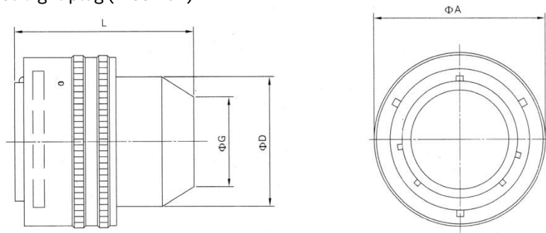
Straight plug (MS3116P)
