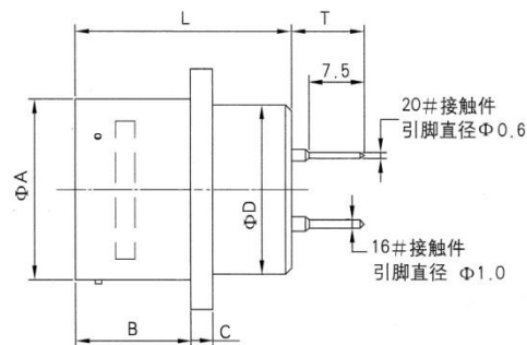
Box square flange receptacle (MS3112B)
